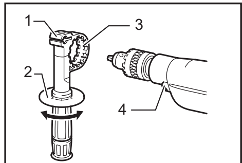
► 1. Grip base 2. Side grip (auxiliary handle) 3. Teeth 4. Protrusions
